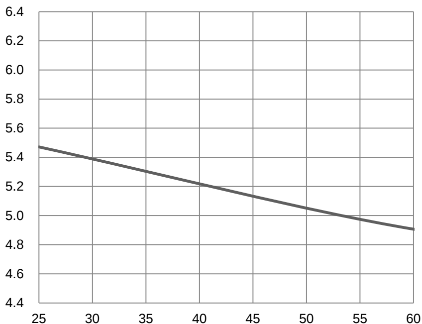
Fig 7. Ambient Temperature vs. Forward Voltage, I_F=120\text{mA}
