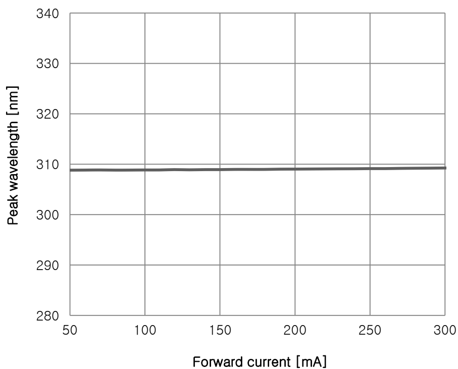
Fig 4. Forward Current vs. Peak Wavelength
