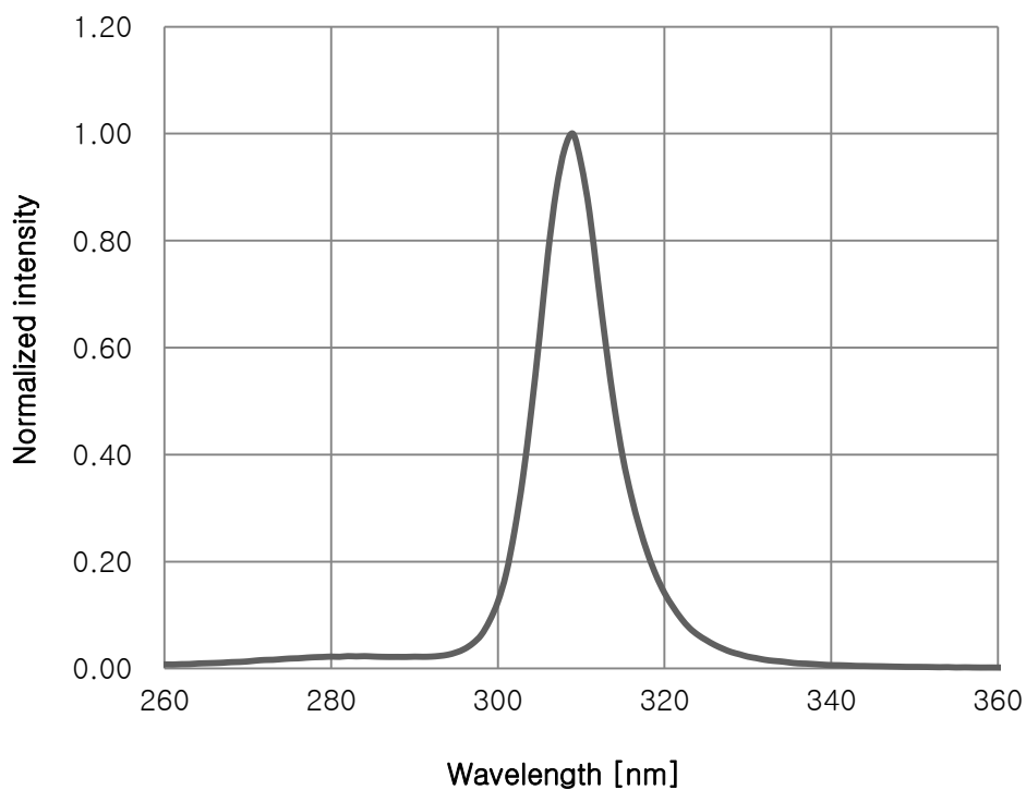
Fig 1. Spectrum, T_a=25^{\circ}\text{C} , I_F=120\text{mA}
