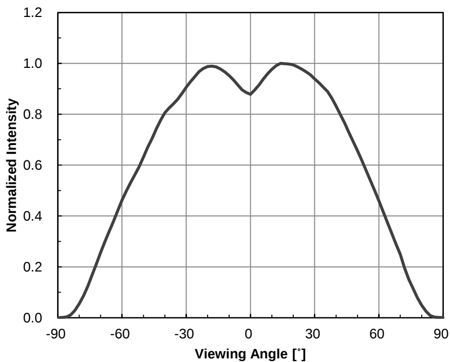
Fig 8. Typical Spatial Distribution, I_F=120\text{mA}
