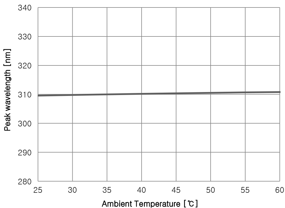
Fig 6. Ambient Temperature vs. Peak Wavelength, I_F=120\text{mA}
