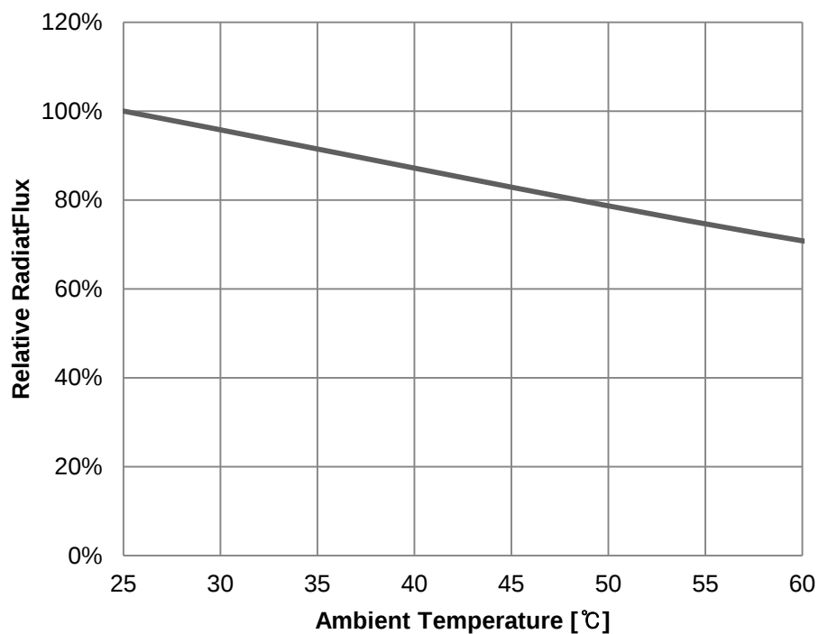
Fig 5. Ambient Temperature vs. Relative Radiant Flux, I_F=120\text{mA}
